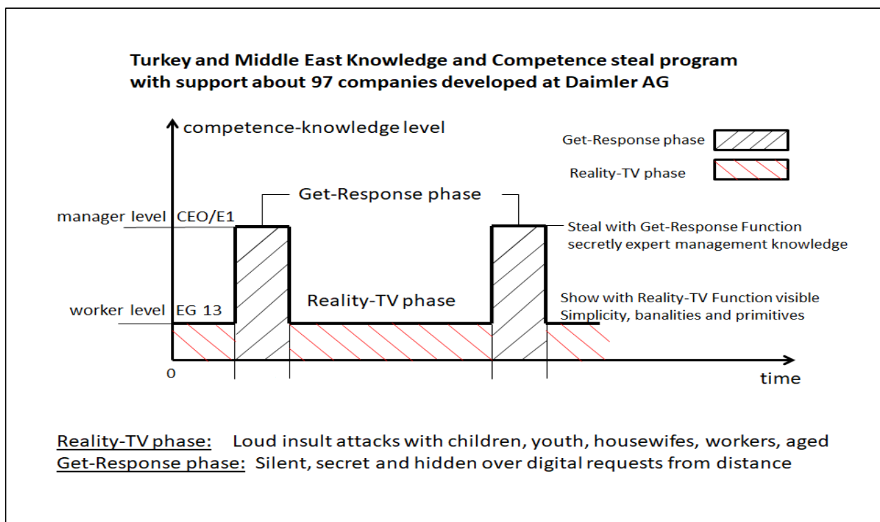
Chart 32: Symmetric/antisymmetric spying phases, time units are variable
